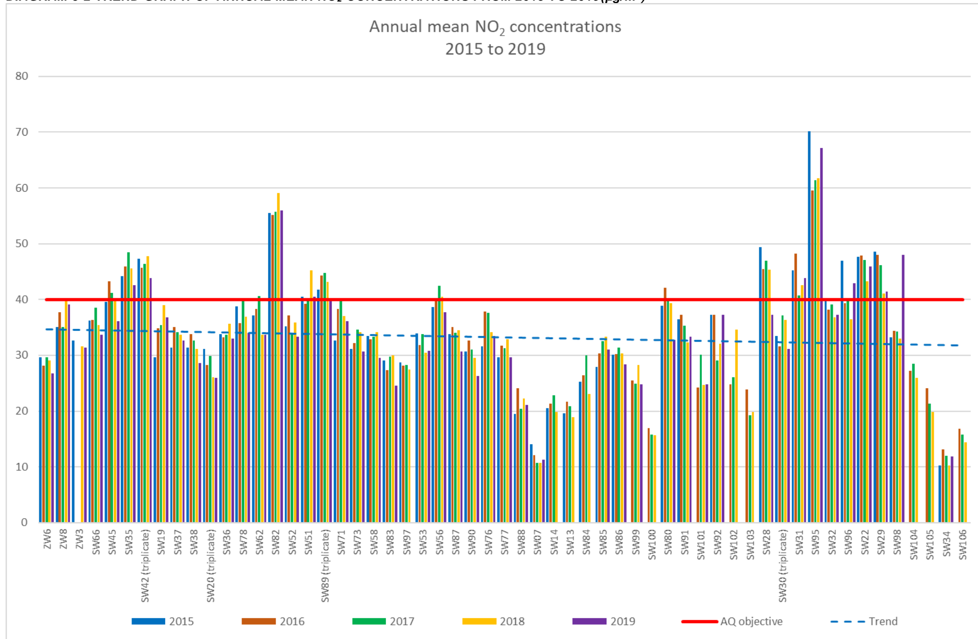
DIAGRAM 5-2 TREND GRAPH OF ANNUAL MEAN NO 2 CONCENTRATIONS FROM 2015 TO 2019(µg/m 3 )
