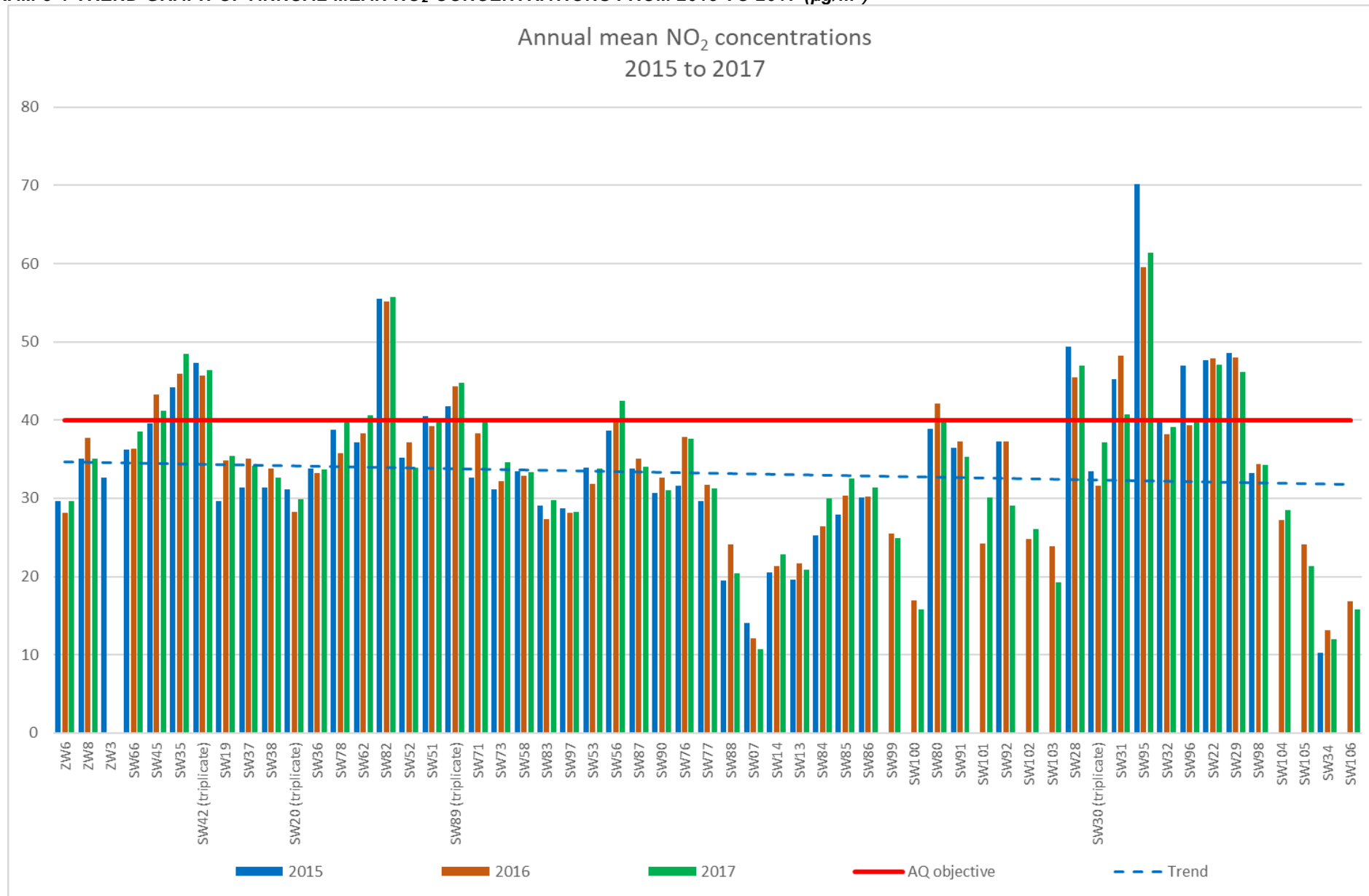
DIAGRAM 5-1 TREND GRAPH OF ANNUAL MEAN NO 2 CONCENTRATIONS FROM 2015 TO 2017 ( \mu\text{g}/\text{m}^3 )
